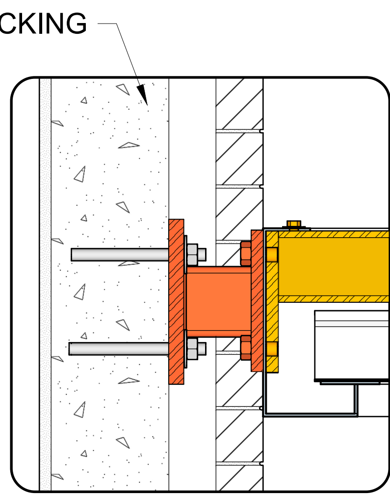
BRYN-MAWR (CHEMICAL ANCHOR) OPTION
