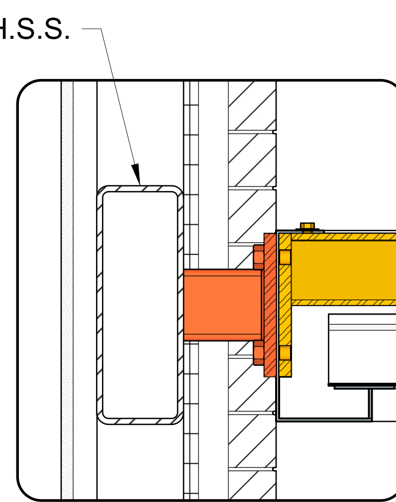
BRYN-MAWR (WELD TYPE) OPTION
